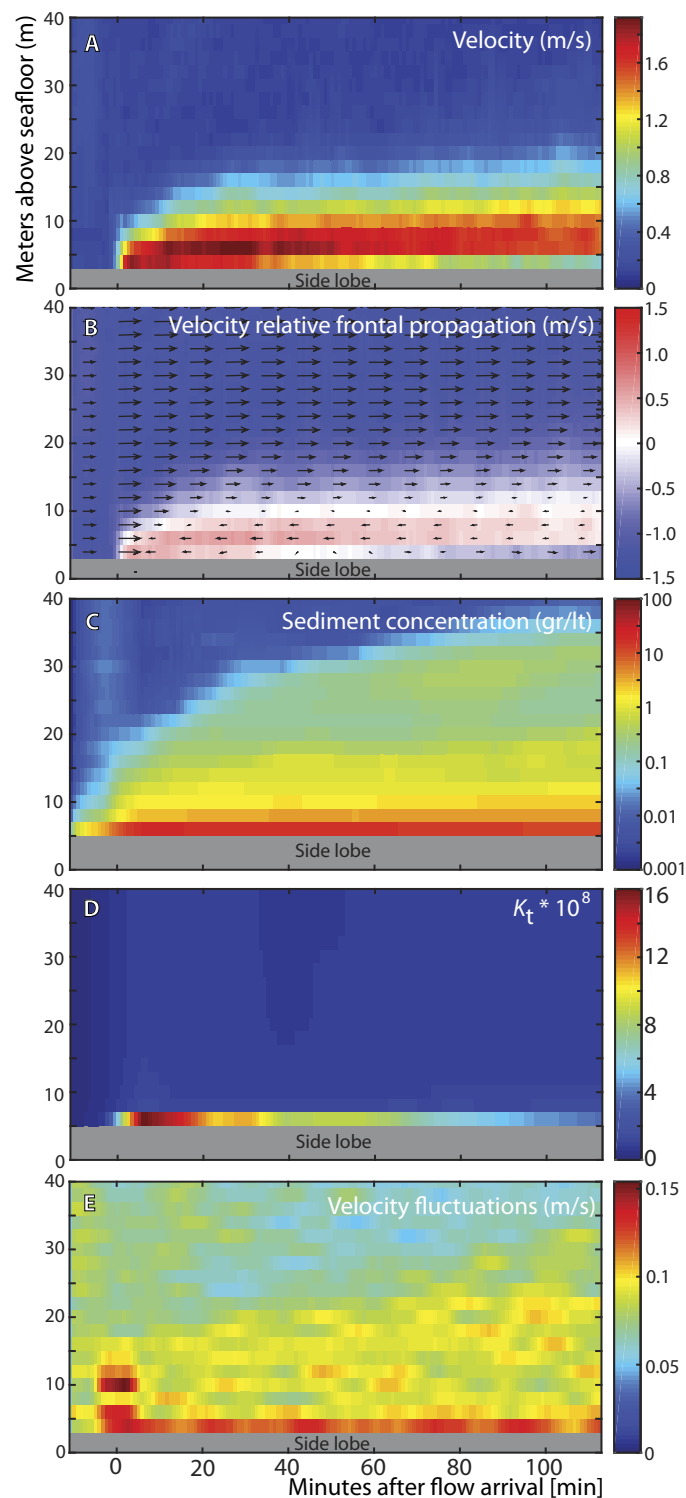
Fig. 5. Structure of the frontal-cell during the first 120 min of the flow. (A) Horizontal flow velocity. Side lobe interference area (see Materials and Methods) is covered by the gray box. (B) Velocity relative to the flow front propagation velocity (which is here fixed at 1.35 m/s). (C) Sediment concentration as derived from the acoustic inversion. (D) Variation of the calibration constant ( K_t ) is used to indicate either grain size variation or higher sediment concentrations (see Materials and Methods). (E) Velocity fluctuations.
