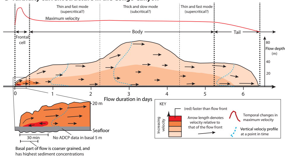
Fig. 4. Turbidity current structure in laboratory experiments and in the Congo Canyon. Structure is shown by temporal changes in velocity measured at one spatial position, with red solid line denoting highest flow velocities. (A) Typical laboratory experiment with a finite-volume (surge-like) release (13–16) or previous oceanographic measurements (30–34); more sustained input would produce a better developed body. Arrows denote relative movement of sediment-laden fluid with respect to the flow front, with flow front velocity thus subtracted from measured velocities. The arrows show whether the body feeds the head. Temporal changes in maximum flow velocity are shown by red lines, and velocity profile shapes are shown by blue dotted lines. (B) Turbidity current structure in the Congo Canyon.
